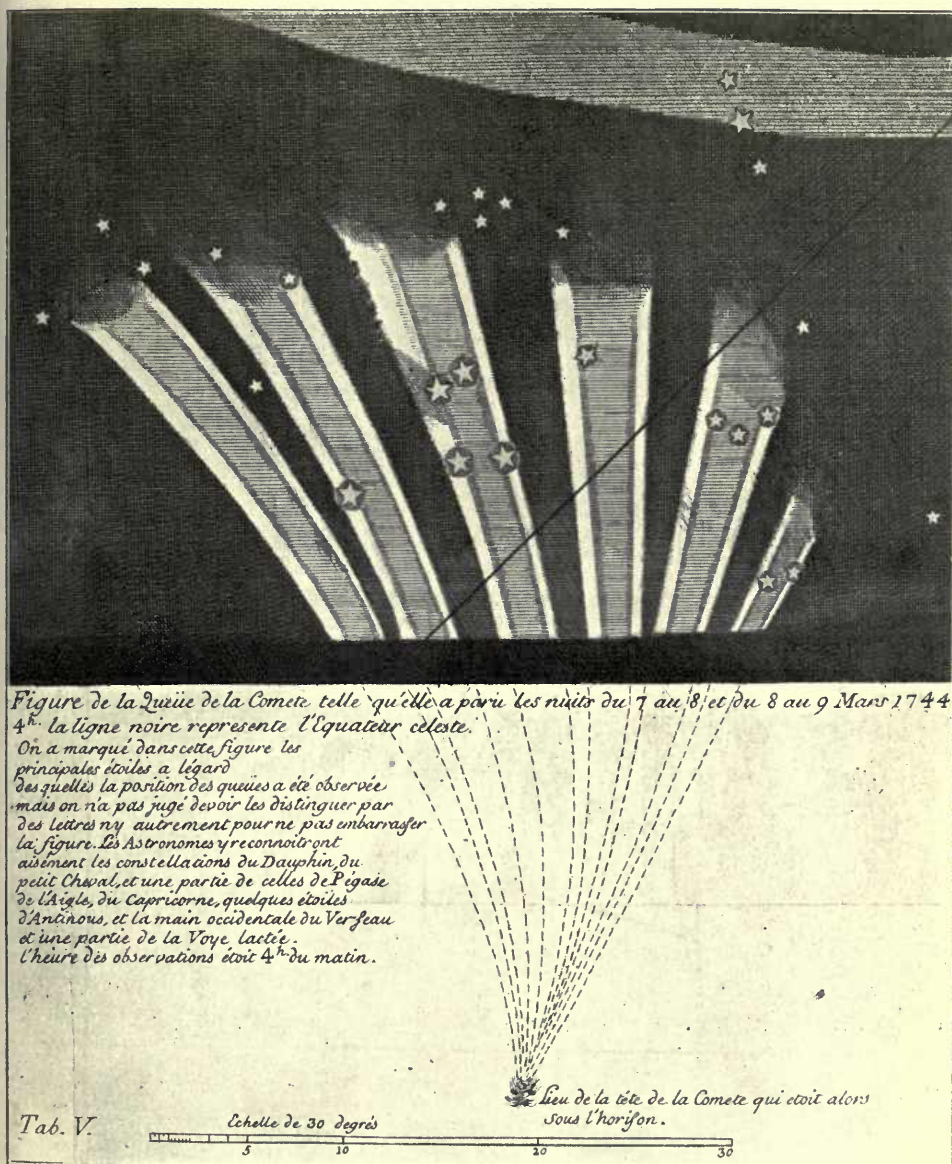
THE GREAT COMET OF 1744. March 7.
