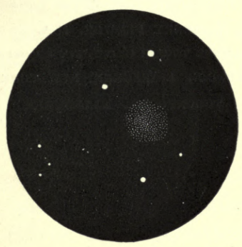
DISCOVERY FIELD OF BROOKS'S COMET OF 1895 (iii.).
