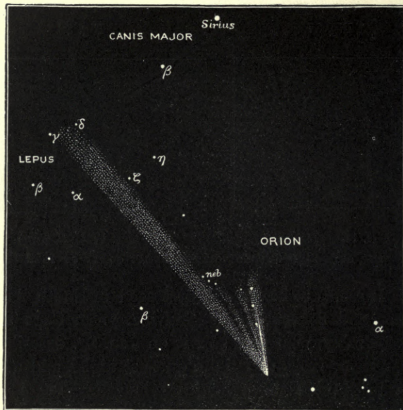
THE GREAT COMET OF 1901 (ii.) ON MAY 12.
