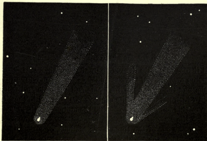
July 23. July 26. THE BROOKS-BORELLY COMET OF 1900 (ii.). (Drawn by W. R. Brooks.)
