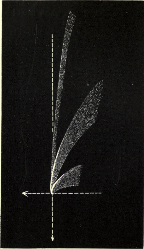
BREDICHIN'S THREE TYPES OF COMET TAILS.
