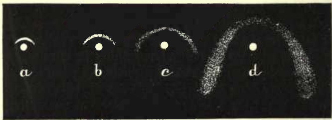
IDEAL DIAGRAM OF THE FORMATION AND DEVELOPEMENT OF "ENVELOPES" IN THE HEAD OF A COMET.
