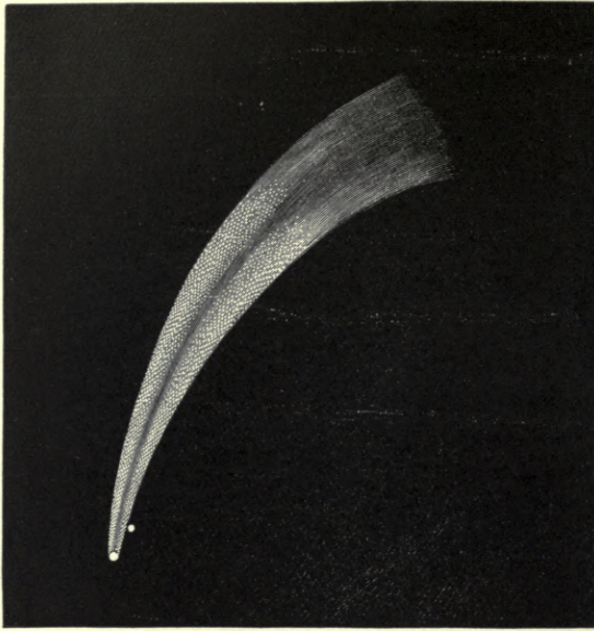
DONATI'S COMET, 1858, PASSING ARCTURUS ON OCT. 5.
