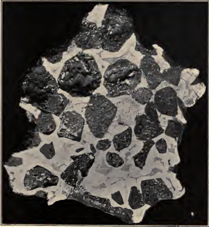
Etched section of South Bend meteorite, showing arrangement of nickel-iron and chrysolite. The light portions are nickel-iron, the dark chrysolite, \times \frac{5}{8} .
